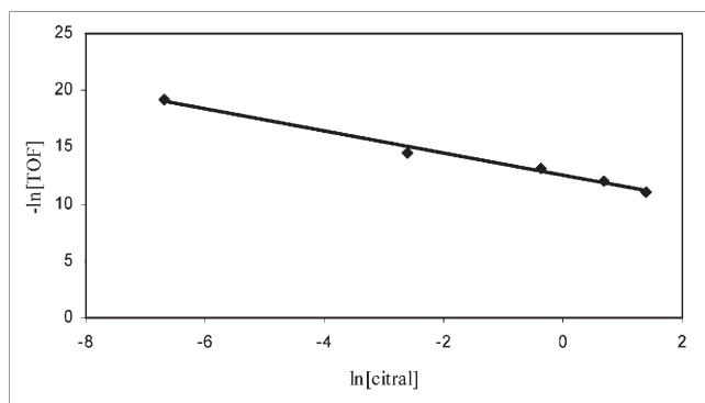
Figure 5. Reaction order with respect to the citral concentration. Reaction conditions: T=70^{\circ}\text{C} ; P_{\text{CO}_2}=14\text{ MPa} ; P_{\text{H}_2}=4\text{ MPa} ; amount of catalyst = 0.1 g.
