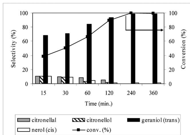
Figure 2. Effect of time variation on conversion and selectivity. Reaction conditions: T = 70^{\circ}\text{C} ; P_{\text{CO}_2} = 14 \text{ MPa} ; P_{\text{H}_2} = 4 \text{ MPa} ; amount of catalyst = 0.1 g; reactant = 6.24 mmol.
