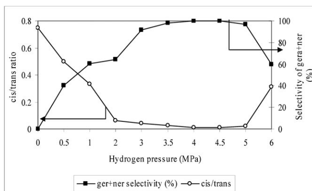
Figure 3. cis:trans Ratio and selectivity to geraniol ( trans )+nerol ( cis ) as a function of H 2 pressure. Reaction conditions: T = 70^{\circ}\text{C} ; P_{\text{CO}_2} = 14 \text{ MPa} ; reaction time = 4 h; amount of catalyst = 0.1 g; reactant = 6.24 mmol.
