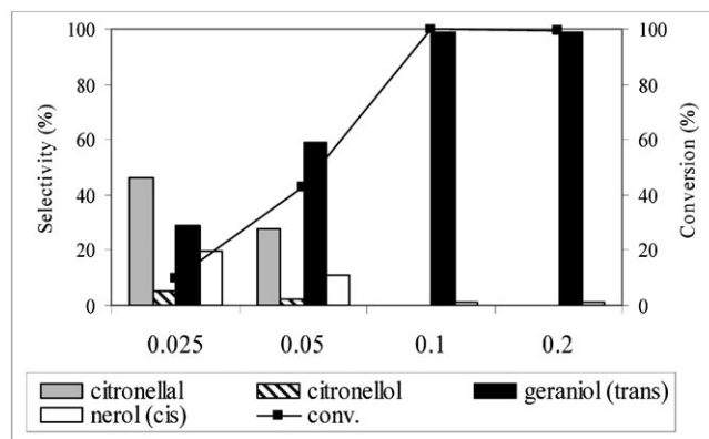
Figure 6. Effect of the catalyst amount on the hydrogenation of citral in scCO 2 . Reaction conditions: T=70^{\circ}\text{C} ; P_{\text{CO}_2}=14\text{ MPa} ; P_{\text{H}_2}=4\text{ MPa} ; reaction time = 4 h; reactant = 6.24 mmol.
