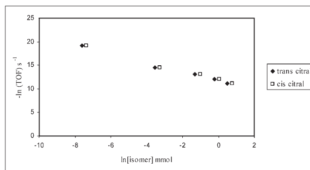
Figure 8. Dependence of hydrogenation rate with each isomer concentration. Reaction conditions: T = 70^\circ\text{C} ; P_{\text{CO}_2} = 14 \text{ MPa} ; P_{\text{H}_2} = 4 \text{ MPa} ; amount of catalyst = 0.1 g; reactant = 6.24 mmol.
