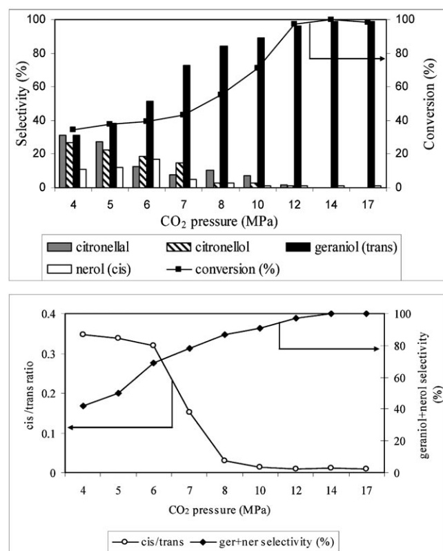
Figure 1. (top) Effect of CO 2 pressure on the conversion and the product distribution of citral hydrogenation. (bottom) Variation of cis/trans ratio with the selectivity of unsaturated alcohol. Reaction conditions: T = 70 °C; reaction time = 4 h; P H 2 = 4 MPa; amount of catalyst = 0.1 g; reactant = 6.24 mmol.
