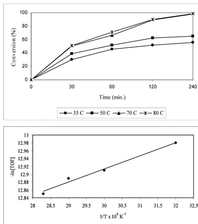
Figure 4. (top) Effect of temperature on citral conversion with time. (bottom) Arrhenius plot. Reaction conditions: P CO 2 = 14 MPa; P H 2 = 4 MPa; amount of catalyst = 0.1 g; reactant = 6.24 mmol.
