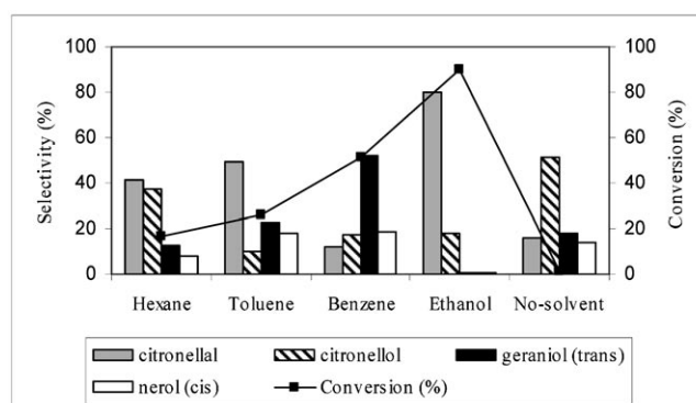
Figure 7. Effect of organic solvents and no solvent conditions on the conversion and selectivity of citral hydrogenation. Reaction conditions: T=70^{\circ}\text{C} ; P_{\text{CO}_2}=14\text{ MPa} ; P_{\text{H}_2}=4\text{ MPa} ; time = 4 h; organic solvent = 10 mL; amount of catalyst = 0.1 g; reactant = 6.24 mmol.
