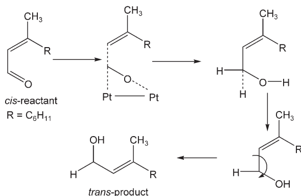
Scheme 2. Probable reaction path of cis to trans isomerization during citral hydrogenation in scCO 2 .
