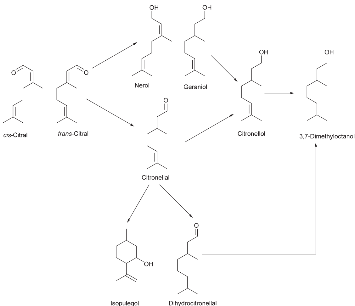
Scheme 1. Probable reaction pathway of citral hydrogenation in supercritical carbon dioxide.
